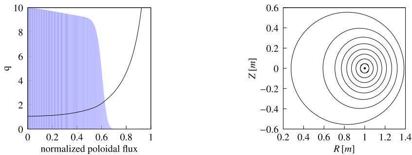
(a) The flux quantities safety factor q (solid line) and the pressure p (shaded, normalized to value at magnetic axis).
